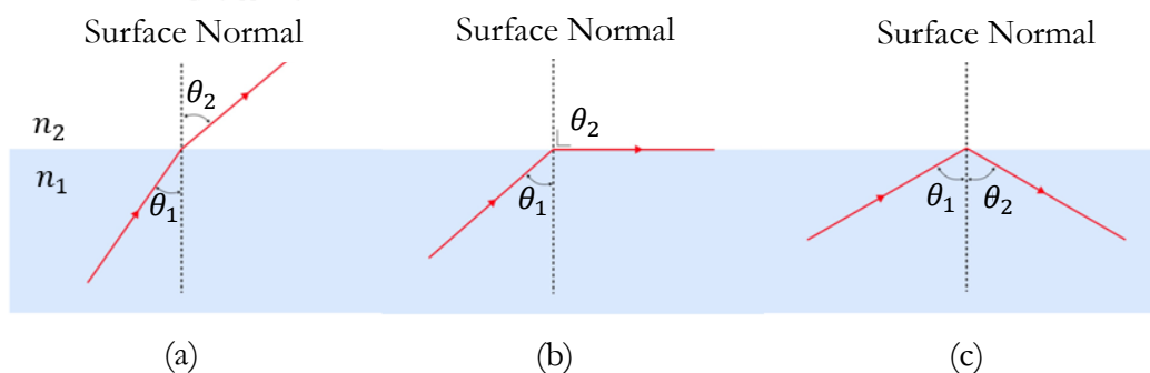
Figure 2. Light propagation from a medium with a higher refractive index toward a medium with a lower refractive index: (a) when \theta_1 < \theta_c , the incident ray is refracted into the second medium; (b) when \theta_1 = \theta_c , the ray does not penetrate the second medium but travels parallel to the boundary between the two media; (c) when \theta_1 > \theta_c , the incident ray undergoes total internal reflection with the angle of reflection equal to the angle of incidence.
