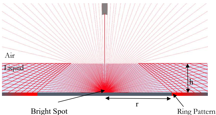
Figure 4. Formation of the light ring pattern on the base of the liquid as a result of total internal reflection at the liquid-air interface.
